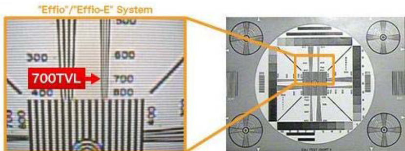
True captured image by "Effio" with 960H CCD image sensor. Resolution test chart
